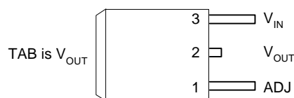
Front View APL1085 TO-263 Package
